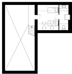
The Coal House - First Floor
