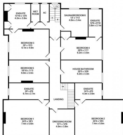
1ST FLOOR
